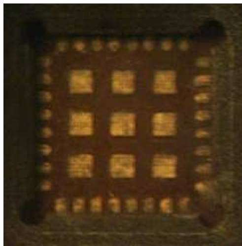
Figure 21 Socket appearance after the last stage of cycling (before cleaning)
