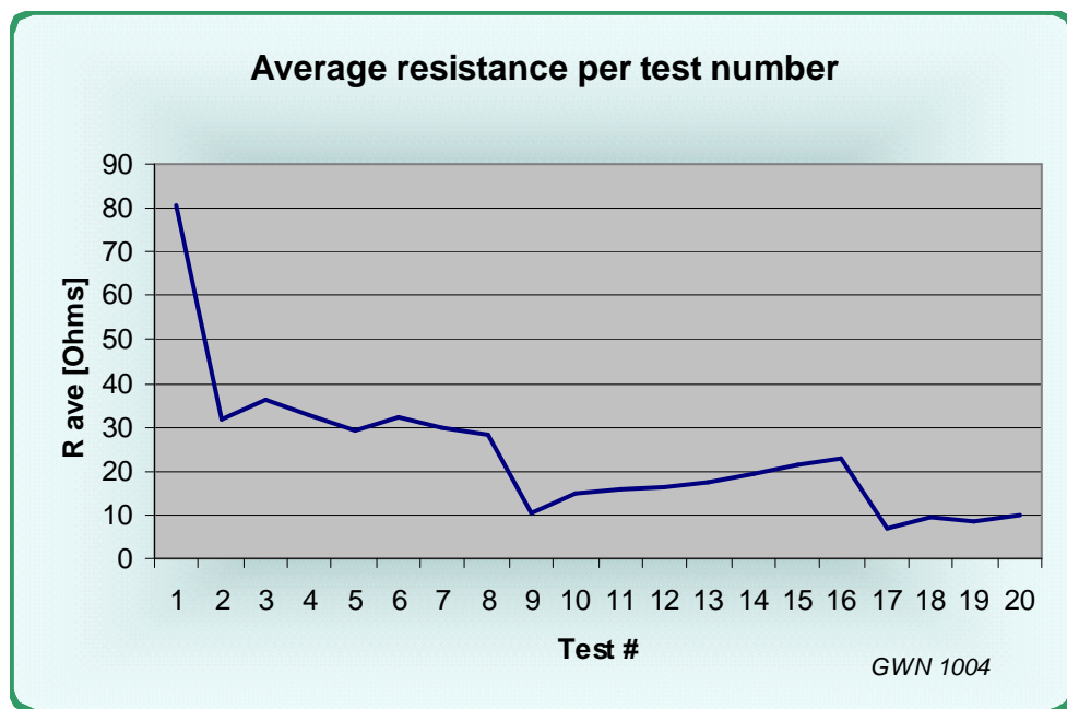
Figure 10 Contact resistance as a function of cycle number
