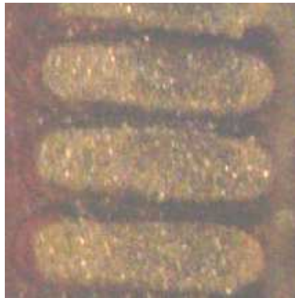
Figure 21 Contact appearance after the last stage of cycling (before cleaning)
