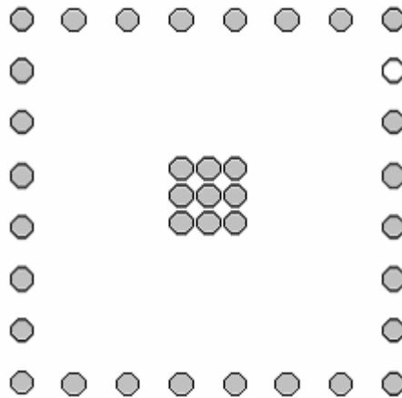
Figure 1 CSP microstrip socket test arrangement; the marked pin is driven
