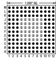
108 Pins – Footprint #12024
