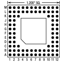
84 Pins – Footprint #12012
