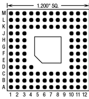
109 Pins – Footprint #12002
