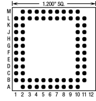
72 Pins – Footprint #12016
