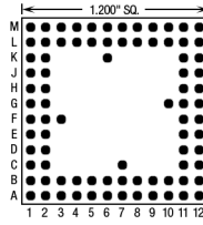
84 Pins – Footprint #12011
