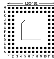
80 Pins – Footprint #12027
