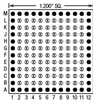
44 Pins – Footprint #12017
