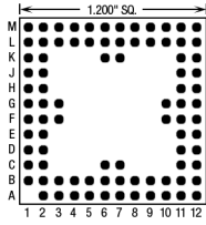
88 Pins – Footprint #12009
