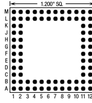
80 Pins – Footprint #12015
