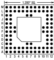
89 Pins – Footprint #12006
