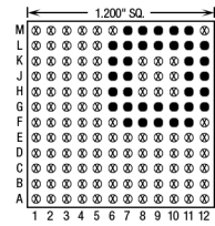
36 Pins – Footprint #12020
