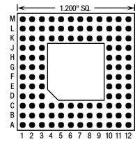
108 Pins – Footprint #12004
