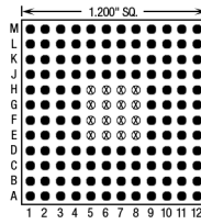
128 Pins – Footprint #12023
