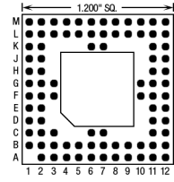
88 Pins – Footprint #12008
