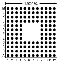
128 Pins – Footprint #12025
