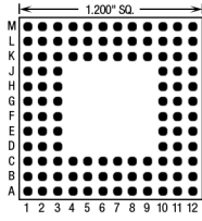
108 Pins – Footprint #12005
