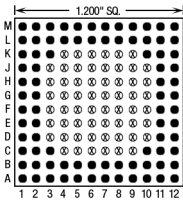
84 Pins – Footprint #12022
