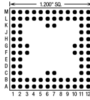
89 Pins – Footprint #12007
