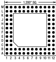
80 Pins – Footprint #12014
