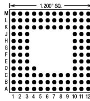
109 Pins – Footprint #12003
