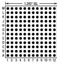
144 Pins – Footprint #12001
