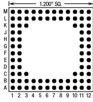
84 Pins – Footprint #12013
