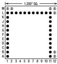
31 Pins – Footprint #12026
