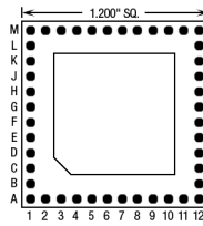
44 Pins – Footprint #12019
