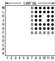
28 Pins – Footprint #12021
