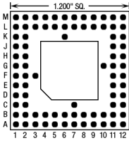
84 Pins – Footprint #12010
