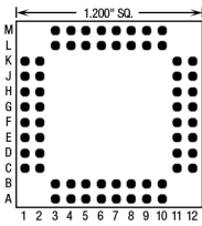
64 Pins – Footprint #12018
