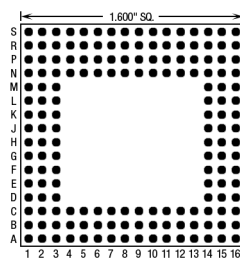
166 Pins – Footprint #16004
