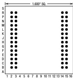
56 Pins – Footprint #16025
