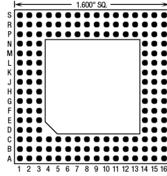
156 Pins – Footprint #16012
