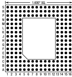
176 Pins – Footprint #16006
