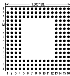
175 Pins – Footprint #16003
