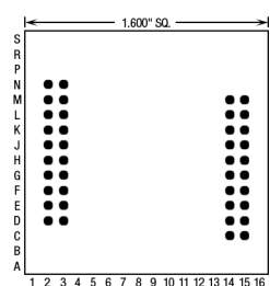
40 Pins – Footprint #16024
