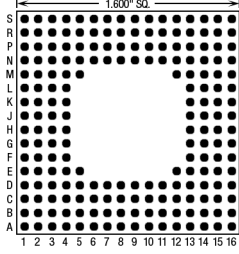
195 Pins – Footprint #16013
