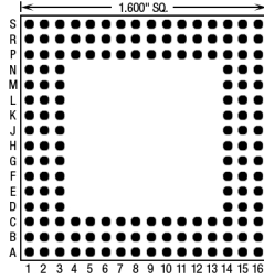
156 Pins – Footprint #16011
