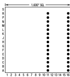
30 Pins – Footprint #16022
