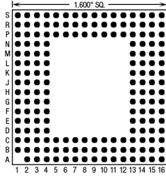
175 Pins – Footprint #16010
