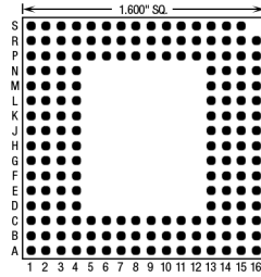
175 Pins – Footprint #16008
