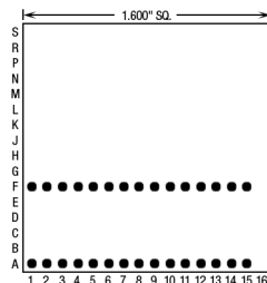
30 Pins – Footprint #16020
