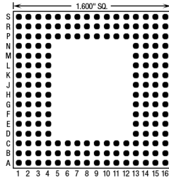
176 Pins – Footprint #16007
