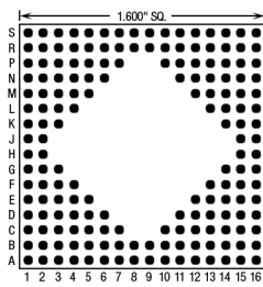
172 Pins – Footprint #16002
