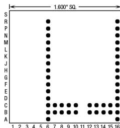
46 Pins – Footprint #16019
