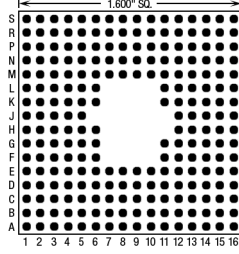
229 Pins – Footprint #16015
