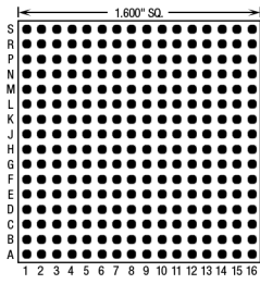
256 Pins – Footprint #16001
