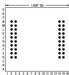
40 Pins – Footprint #16023
