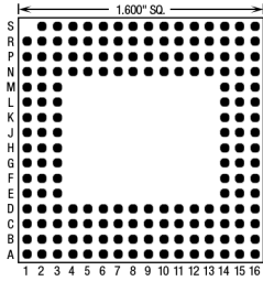
175 Pins – Footprint #16005
