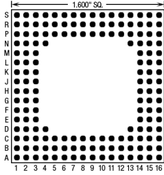
159 Pins – Footprint #16009
