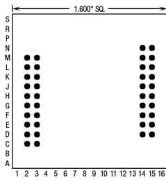
40 Pins – Footprint #16026
