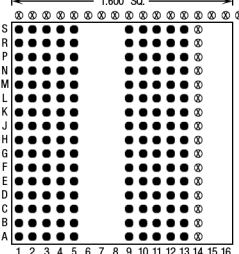
160 Pins – Footprint #16018
