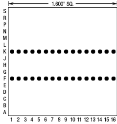
30 Pins – Footprint #16017
