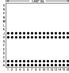
64 Pins – Footprint #16016
