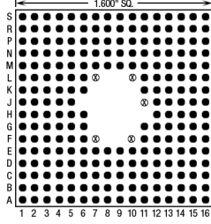
229 Pins – Footprint #16014
