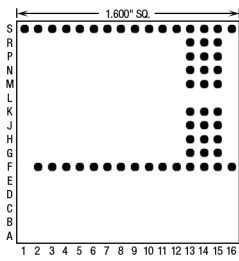
47 Pins – Footprint #16021
