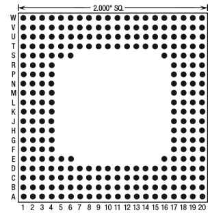
262 Pins – Footprint #20003
