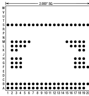
100 Pins – Footprint #20011
