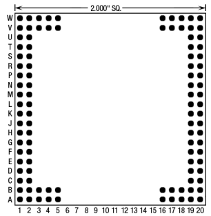
104 Pins – Footprint #20021
