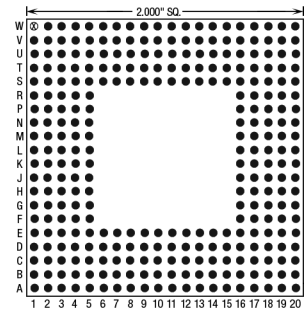
299 Pins – Footprint #20009
