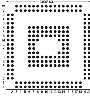
208 Pins – Footprint #20008
