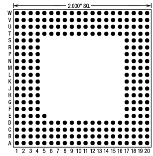
257 Pins – Footprint #20012
