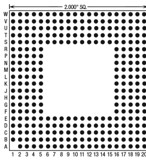
299 Pins – Footprint #20002
