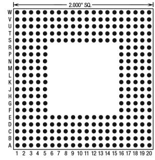
300 Pins – Footprint #20006
