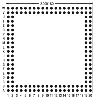
144 Pins – Footprint #20007
