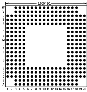
240 Pins – Footprint #20010
