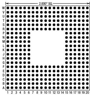
336 Pins – Footprint #20019
