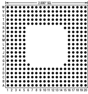
303 Pins – Footprint #20004
