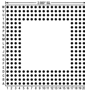
256 Pins – Footprint #20005
