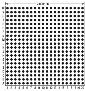
400 Pins – Footprint #20001
