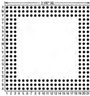
216 Pins – Footprint #21016
