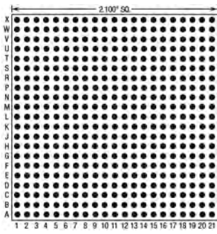
441 Pins – Footprint #21001
