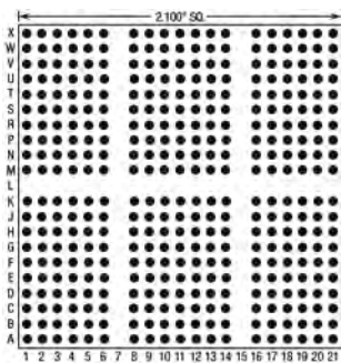
380 Pins – Footprint #21023
