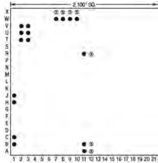
17 Pins – Footprint #21009
