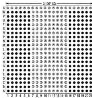
240 Pins – Footprint #21014
