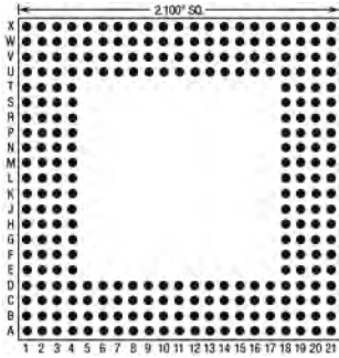
237 Pins – Footprint #21004
