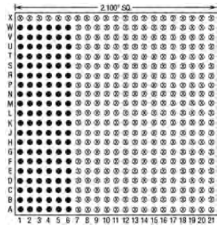
120 Pins – Footprint #21012
