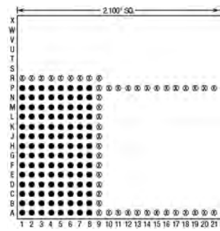
112 Pins – Footprint #21028
