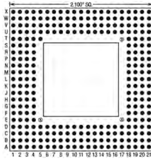
273 Pins – Footprint #21005
