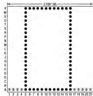
62 Pins – Footprint #21031
