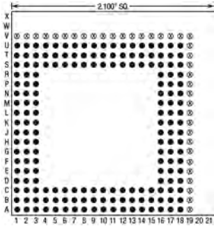
180 Pins – Footprint #21007
