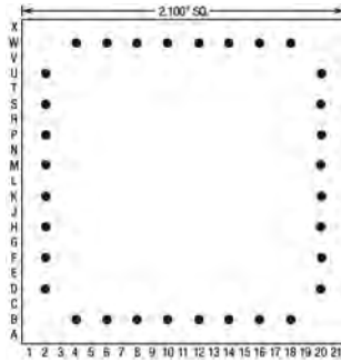
32 Pins – Footprint #21018
