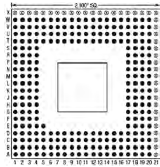
257 Pins – Footprint #21019
