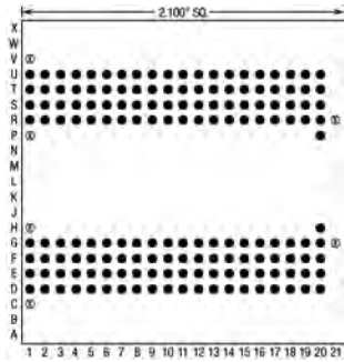
162 Pins – Footprint #21029
