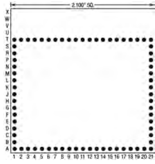
72 Pins – Footprint #21003
