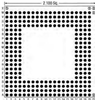
256 Pins – Footprint #21030
