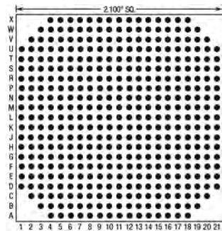
336 Pins – Footprint #21022
