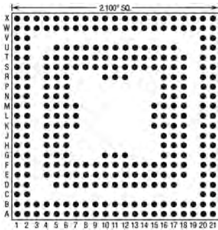
304 Pins – Footprint #21010
