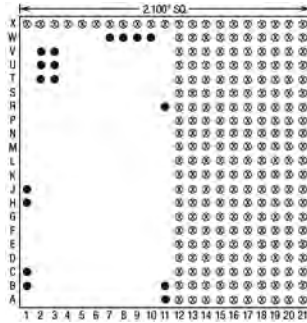
17 Pins – Footprint #21008
