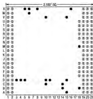
19 Pins – Footprint #21024
