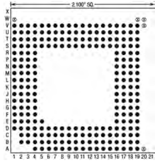
236 Pins – Footprint #21006
