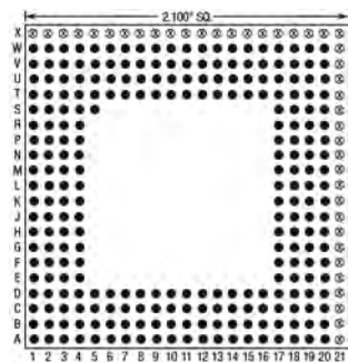
257 Pins – Footprint #21015
