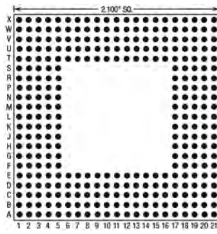
319 Pins – Footprint #21002
