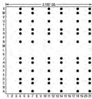
72 Pins – Footprint #21026
