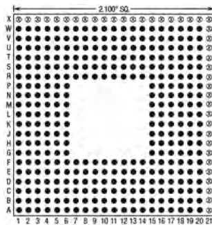
366 Pins – Footprint #21021
