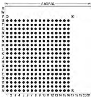
288 Pins – Footprint #21020
