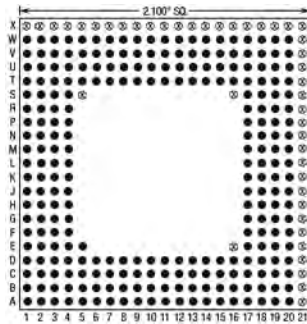
257 Pins – Footprint #21011
