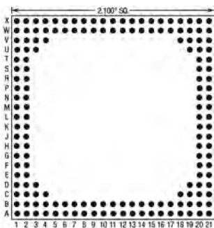
164 Pins – Footprint #21013
