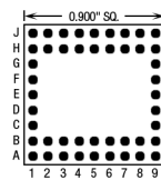
46 Pins – Footprint #09027
