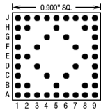
48 Pins – Footprint #09013
