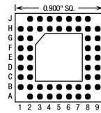
52 Pins – Footprint #09019
