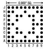
53 Pins – Footprint #09011
