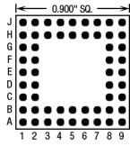
56 Pins – Footprint #09009
