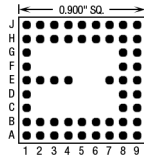
55 Pins – Footprint #09010
