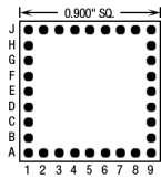
32 Pins – Footprint #09017
