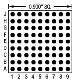
81 Pins – Footprint #09001
