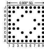
49 Pins – Footprint #09012
