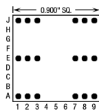
18 Pins – Footprint #09026
