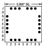
22 Pins – Footprint #09025
