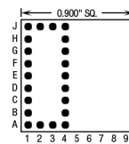
22 Pins – Footprint #09028
