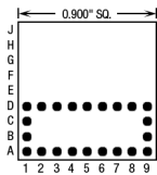
22 Pins – Footprint #09021
