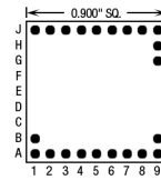
22 Pins – Footprint #09020
