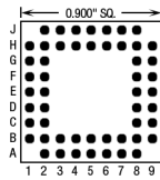
52 Pins – Footprint #09018
