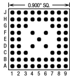
65 Pins – Footprint #09005
