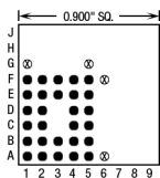
28 Pins – Footprint #09029
